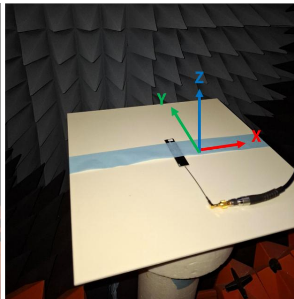
Chamber Setup on 2mm ABS
