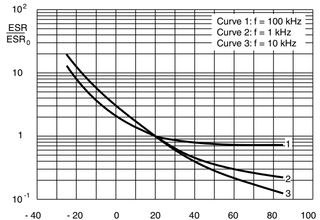
Fig. 6 - Typical multiplier of ESR as a function of ambient temperature at different frequencies
