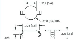
Mounting Detail
