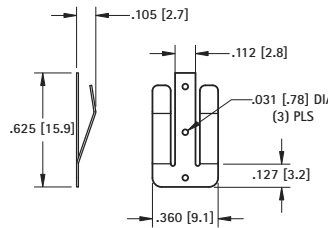
SMT SPRING CONTACT*
