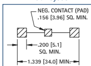
Pad Layout
