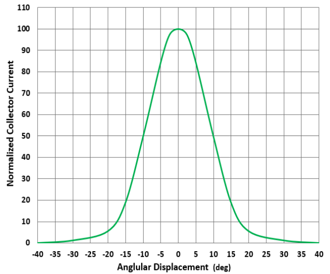
Normalized Collector Current vs Angular Displacement
