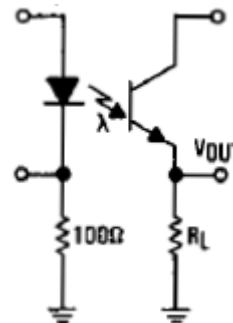
Test Circuit
