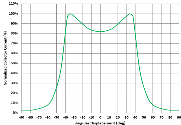
Normalized Collector Current vs Angular Displacement
