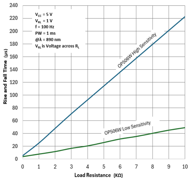
Rise and Fall Times vs Load Resistance
