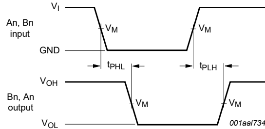
Fig. 5. Propagation delay, data input (An, Bn) to data output (Bn, An)
