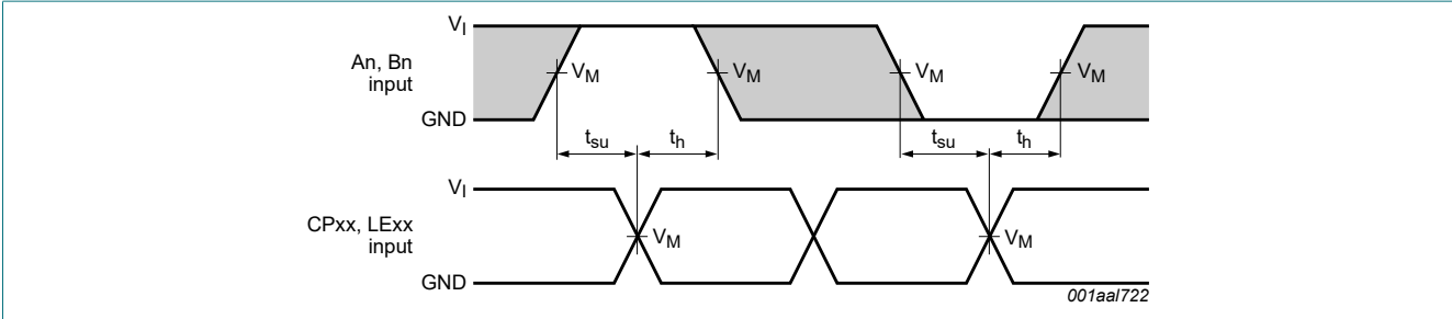
Fig. 8. Data set-up and hold times (An, Bn inputs to LEAB, LEBA, CPAB and CPBA inputs)
