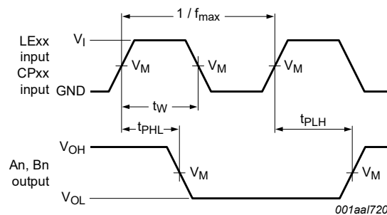
Fig. 6. 3-state output enable and disable times
