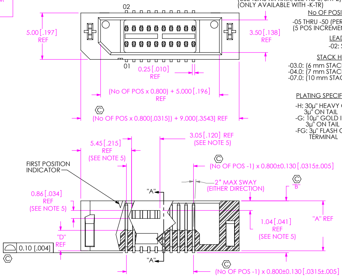
FIG 1 TEM-110-02-03.0-XX-D SHOWN
