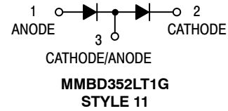
SOT-23 (TO-236) CASE 318
