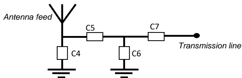
Matching circuit
