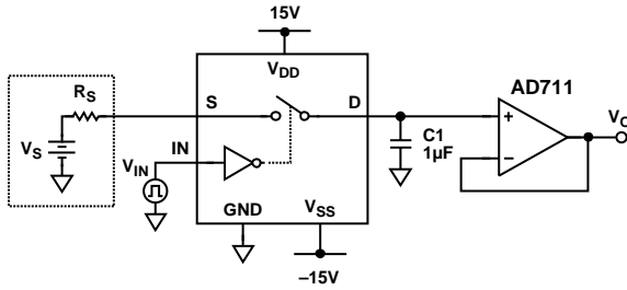
Figure 7. Charge Injection
