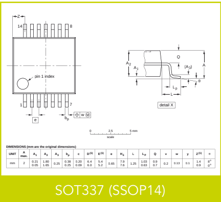
SOT337 (SSOP14)
