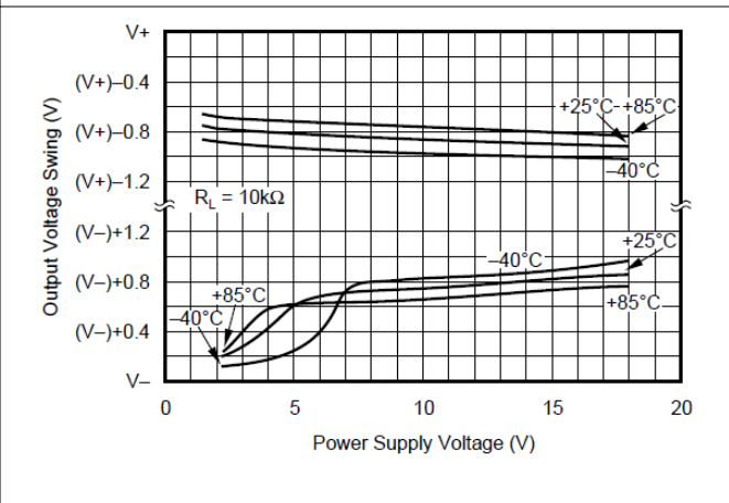
Figure 6-16. Output Voltage Swing vs Power Supply Voltage
