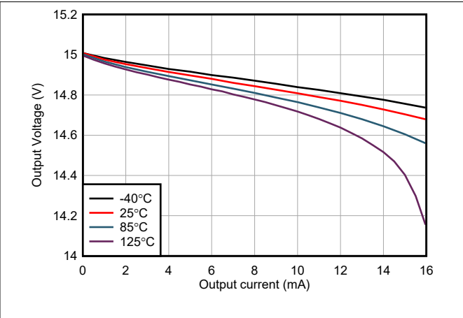
Figure 6-14. Positive Output Voltage Swing vs Output Current
