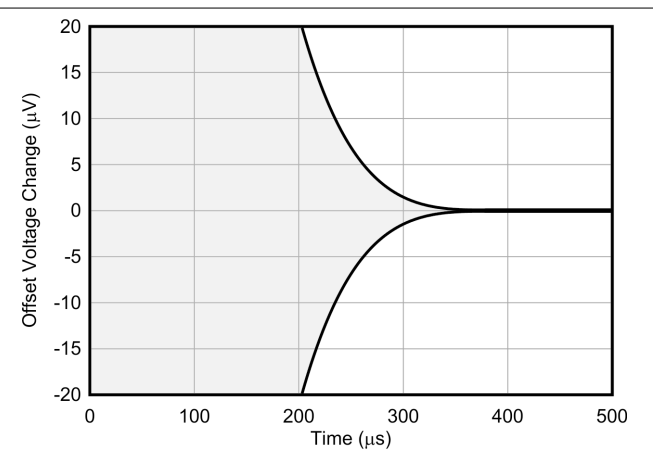
Figure 6-12. Offset Voltage Warm-Up
