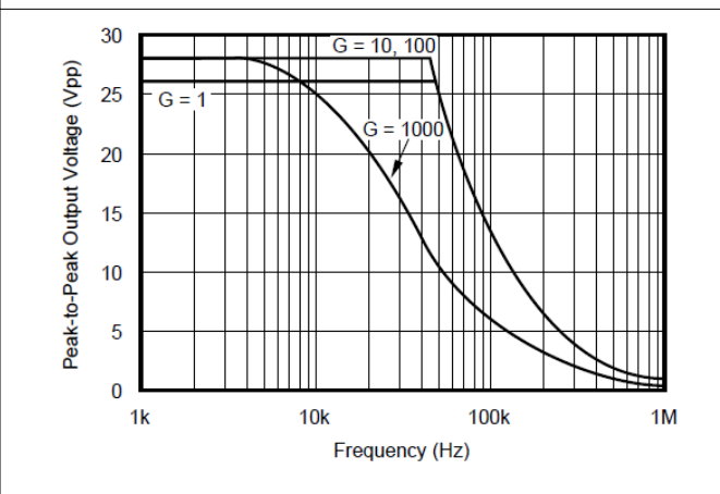
Figure 6-18. Maximum Output Voltage vs Frequency
