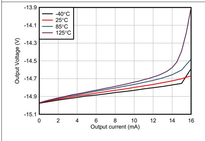
Figure 6-15. Negative Output Voltage Swing vs Output Current
