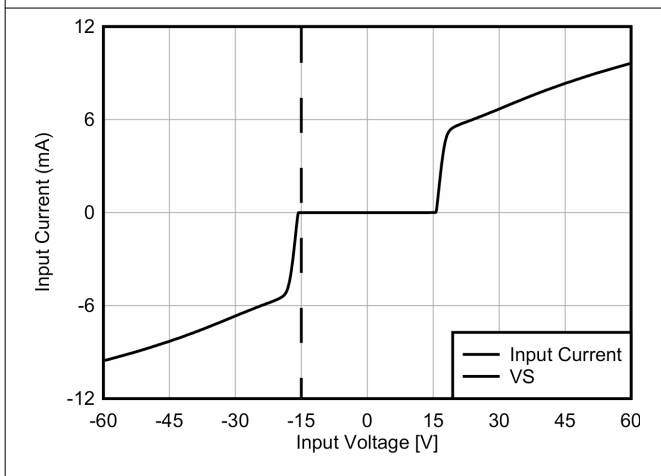
Figure 6-11. Input Overvoltage V/I Characteristics
