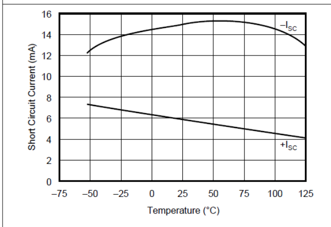
Figure 6-17. Short-Circuit Output Current vs Temperature
