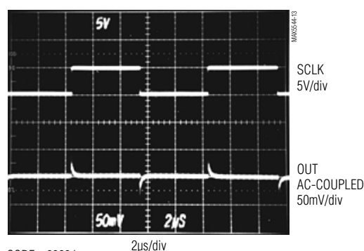
DIGITAL FEEDTHROUGH
