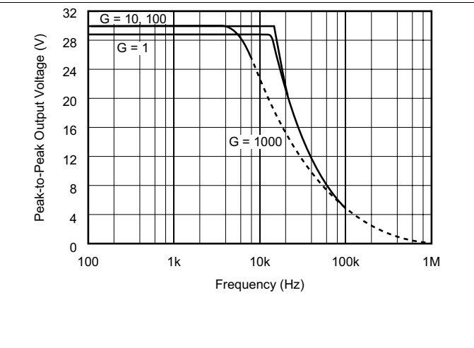
Figure 18. Maximum Output Swing vs Frequency
