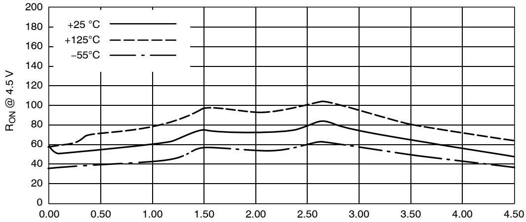
Figure 3. Typical On Resistance, V_{CC} = 4.5 V
