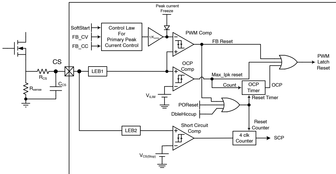
Figure 54. Current Setpoint
