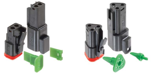
2-Circuit ML-XT System
