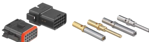
18-Circuit ML-XT System
