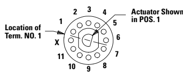
30° Indexing Models Top View
