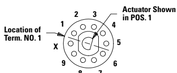
36° Indexing Models Top View
