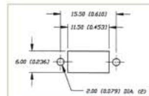
PANEL MOUNT
