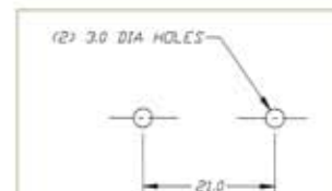
PANEL MOUNT
