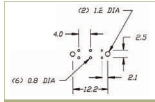
P.C. MOUNTING
