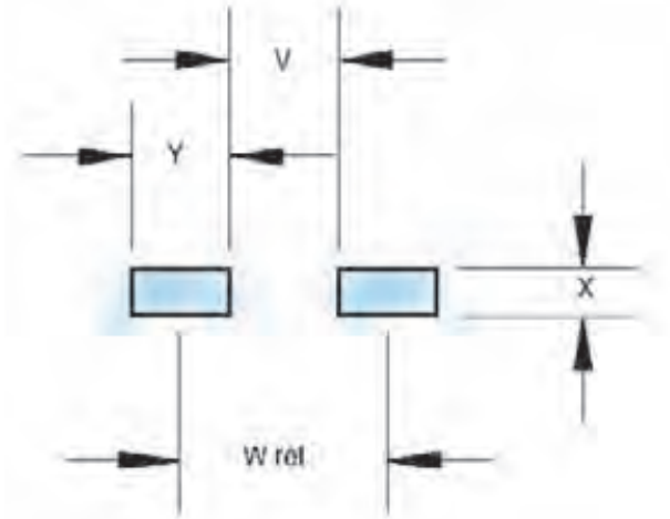
Land Pattern
