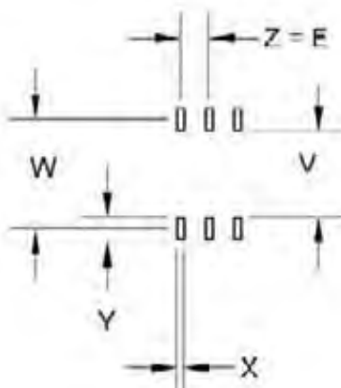
Land Pattern
