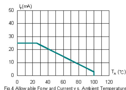
Fig.4 Allowable Forward Current vs. Ambient Temperature
