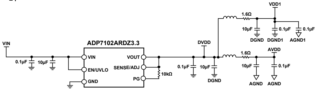
Figure 13. Recommended Circuit and Component Values
