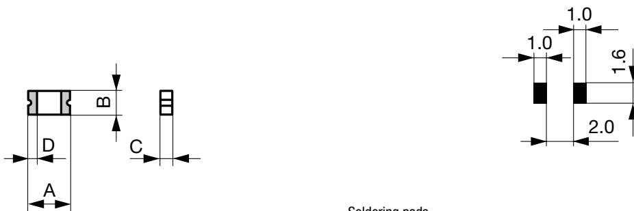
Soldering pads
