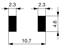
Solder pads PFSM.150.2, PFSM.200.2 and PFSM.250.2
