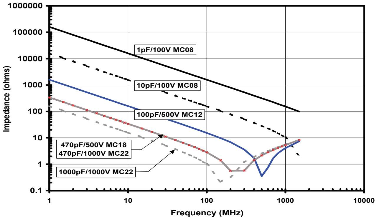
Type MC Typical Impedance vs. Frequency
