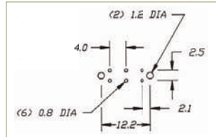
P.C. MOUNTING
