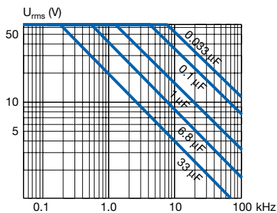
MMK7.5 ... 37.5 100/63
