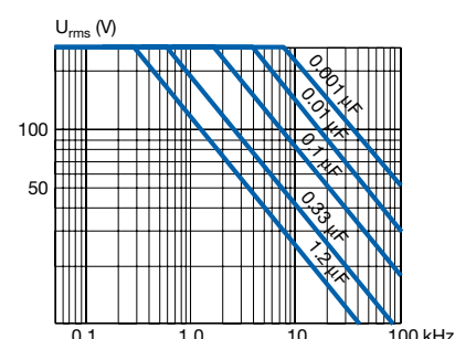
MMK7.5 ... 37.5 1000/250
