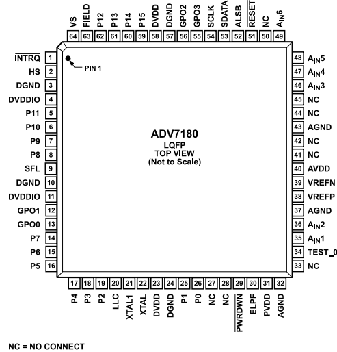
Figure 10. 64-Lead LQFP Pin Configuration
