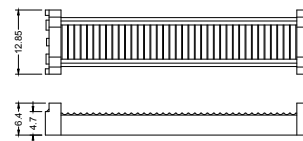
Cable Clamp
