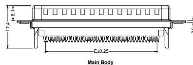
Main Body
