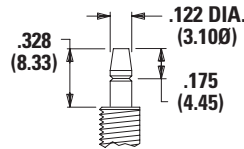
L, L1 Plunger Dimensions
