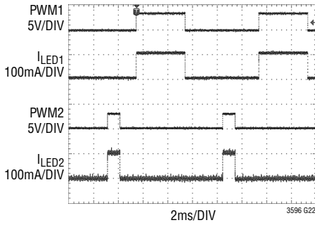
PWM Dimming Waveforms (Nonoverlapping PWM Signals)
