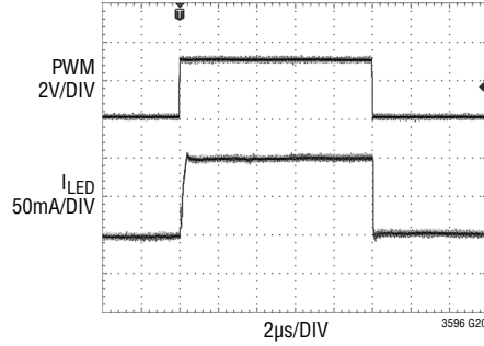
1,000:1 PWM Dimming at 100Hz
