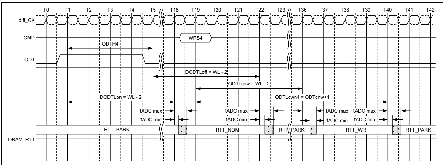
Figure 164 – Synchronous ODT example with BL=4, CWL=9, AL=10, PL=0; DODTLon/off=WL-2=17, ODTcHw=WL-2=17
