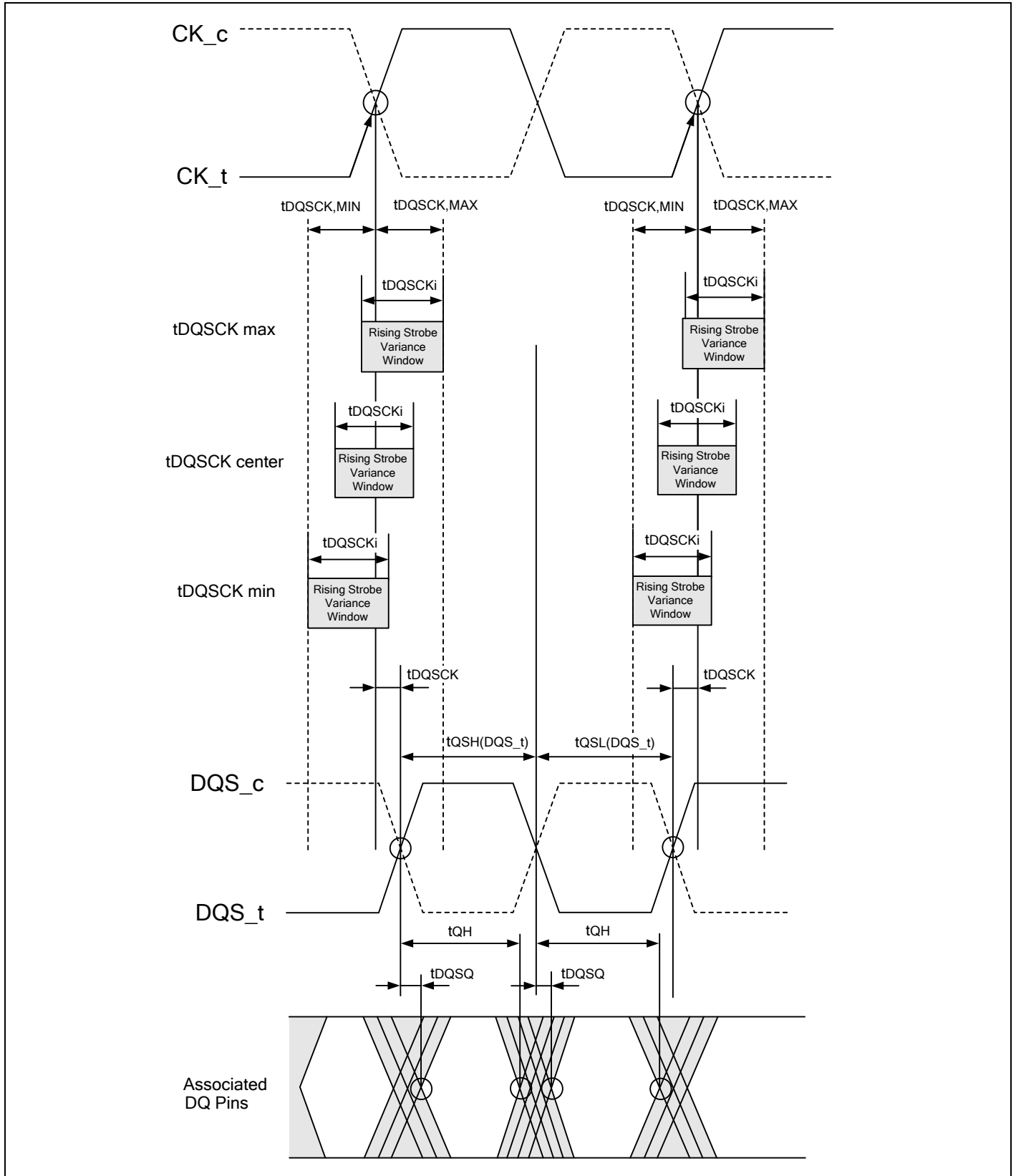
Figure 64 – READ Timing Definition
