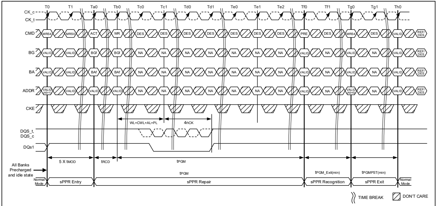
Figure 160 – Fail Row Soft PPR (WR Case)
