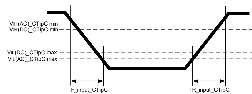
Figure of Input C Slew Rate Definition
