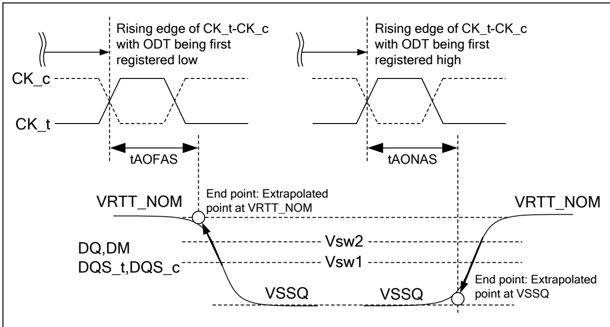
Figure 175 – Definition of t_{AOFAS} and t_{AONAS}
