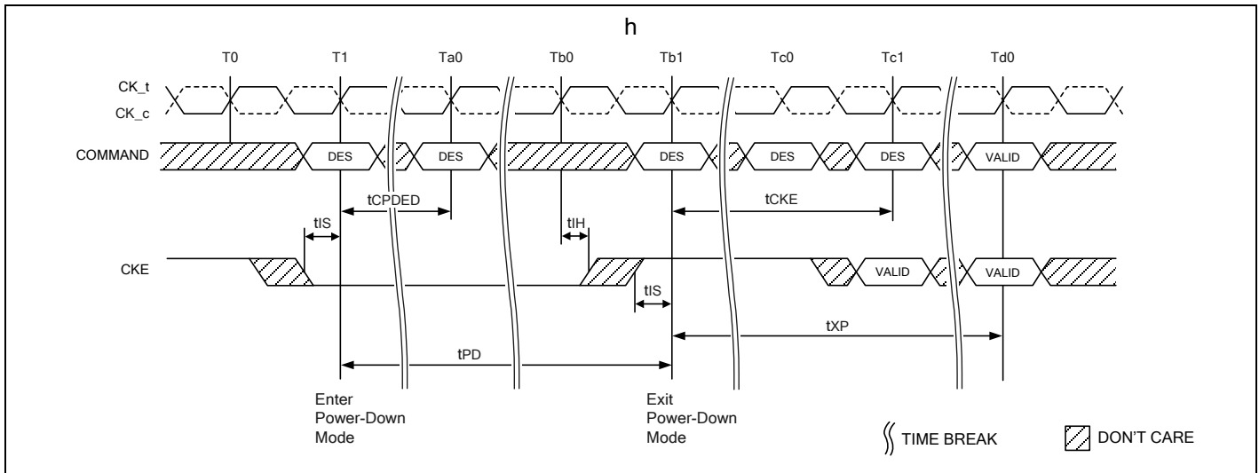
Figure 147 – Precharge Power-Down Entry and Exit
