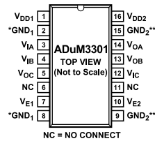
Figure 5. ADuM3301 Pin Configuration
