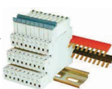
shown on DIN rail with relays and jumpers
