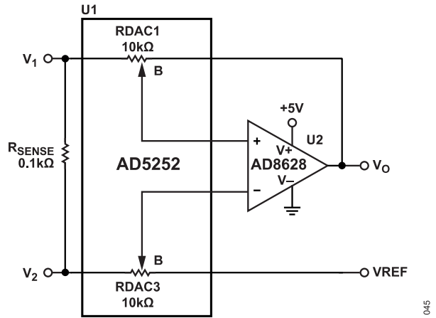
Figure 45. Current-Sensing Amplifier
