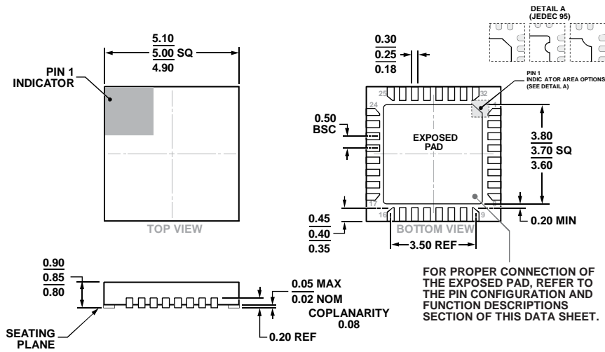
COMPLIANT TO JEDEC STANDARDS MO-220-VHHD-4. Figure 18. 32-Lead Lead Frame Chip Scale Package [LFCSPP] 5 mm x 5 mm Body and 0.85 mm Package Height (HCP-32-1) Dimensions shown in millimeters
