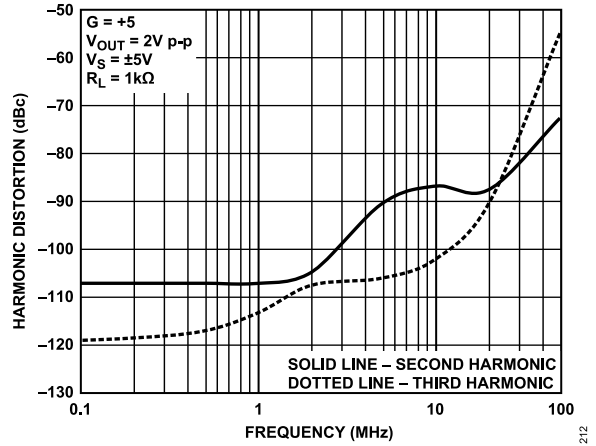
Figure 26. Harmonic Distortion vs. Frequency (LFCSP)
