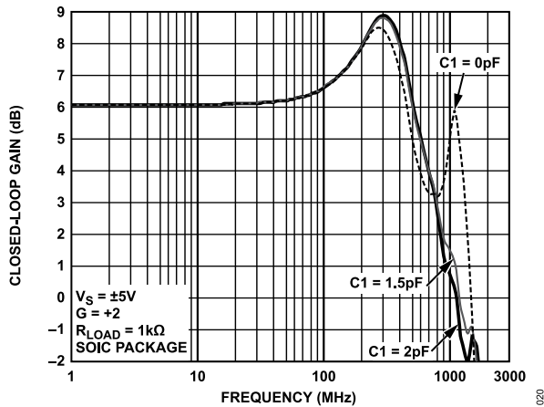
Figure 72. Frequency Response for Various Values of C_1
