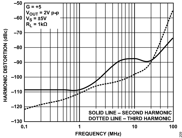
Figure 23. Harmonic Distortion vs. Frequency (SOIC)
