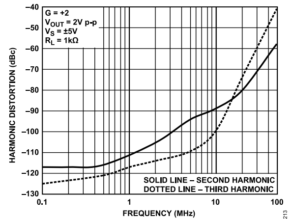
Figure 27. Harmonic Distortion vs. Frequency (LFCSP)
