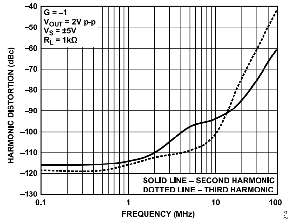
Figure 28. Harmonic Distortion vs. Frequency (LFCSP)
