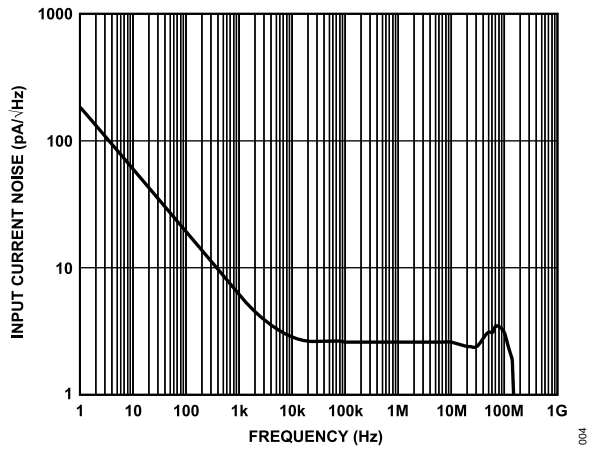
Figure 48. Input Current Noise vs. Frequency ( \overline{DISABLE} = Open )
