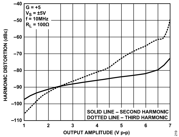
Figure 33. Harmonic Distortion vs. Output Amplitude (LFCSP)
