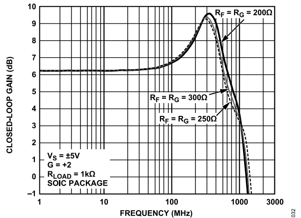
Figure 68. Frequency Response for Various Values of R_F and R_G
