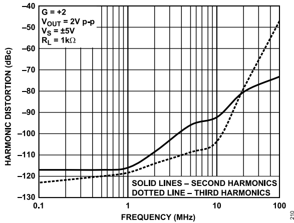
Figure 24. Harmonic Distortion vs. Frequency (SOIC)
