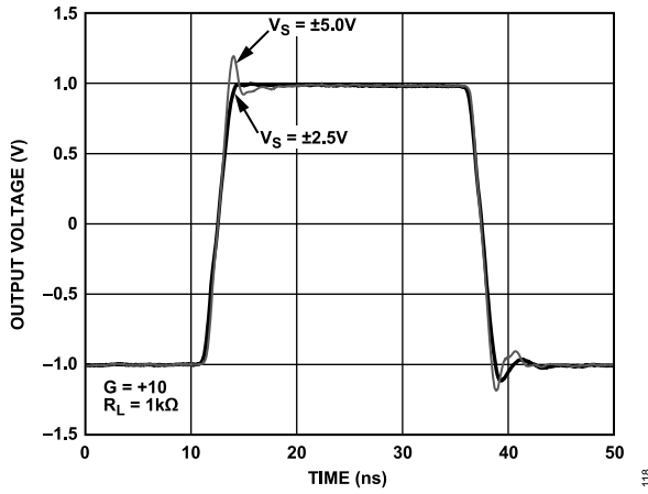
Figure 42. Large Signal Transient Response vs. Supply Voltage (SOIC)
