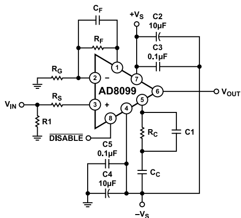
Figure 59. Wideband Noninverting Gain Configuration (SOIC)
