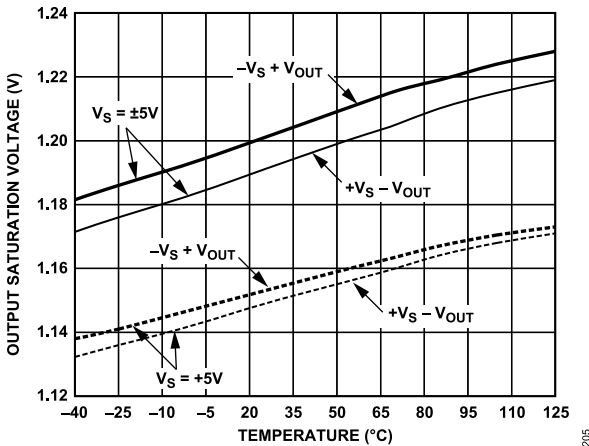
Figure 55. Output Saturation Voltage vs. Temperature
