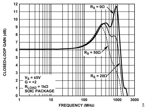
Figure 69. Frequency Response for Various Values of R_S
