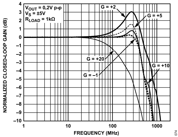
Figure 5. Small Signal Frequency Response for Various Gains (SOIC)
