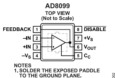
Figure 3. 8-Lead SOIC-EP (RD-8-4)
