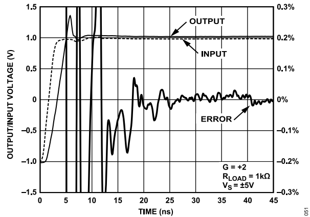
Figure 45. Short Term Settling Time (SOIC)
