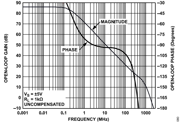
Figure 14. Open Loop Frequency Response
