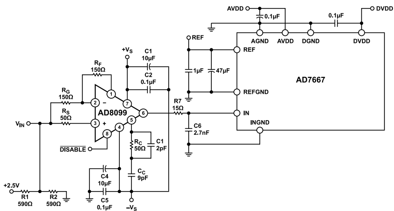
Figure 76. ADC Driver
