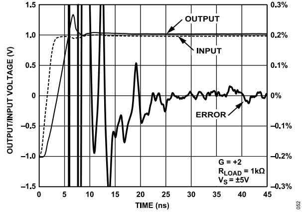
Figure 44. Short Term Settling Time (LFCSP)
