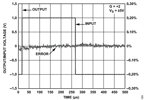
Figure 46. Long Term Settling Time
