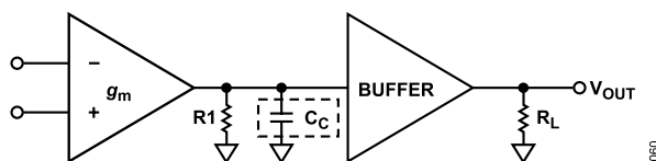
Figure 58. AD8099 Topology
