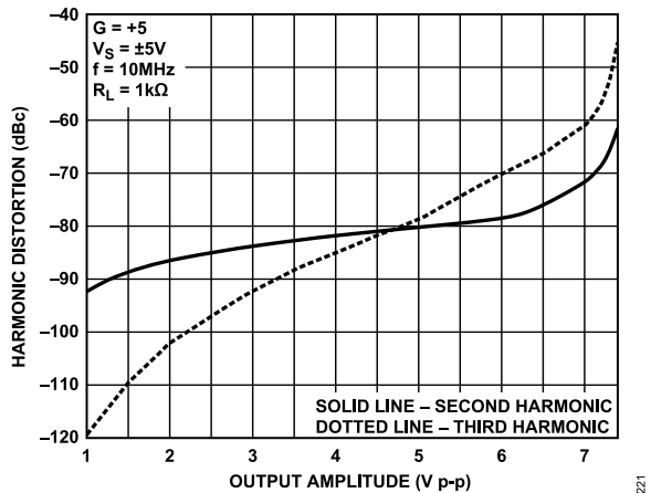
Figure 34. Harmonic Distortion vs. Output Amplitude (LFCSP)
