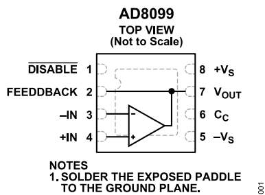
Figure 2. 8-Lead LFCSP (CP-8-13)
