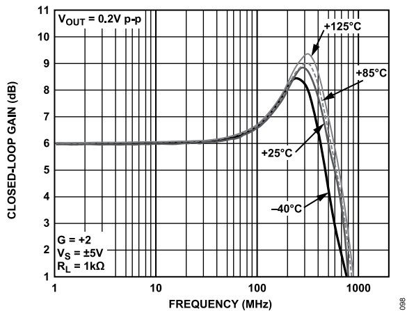
Figure 7. Small Signal Frequency Response for Various Temperatures (SOIC)
