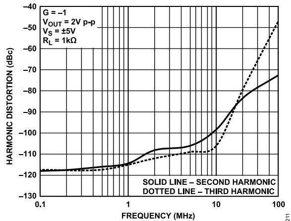
Figure 25. Harmonic Distortion vs. Frequency (SOIC)
