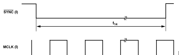
Figure 8. SYNC Pulse Width
