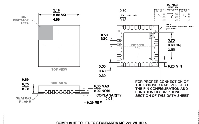
Figure 130. 32-Lead Lead Frame Chip Scale Package [LFCSP] 5 mm x 5 mm Body and 0.75 mm Package Height (CP-32-12) Dimensions shown in millimeters
