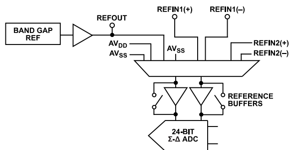
Figure 76. Reference Connections
