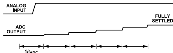
Figure 84. Asynchronous Step Change in the Analog Input
