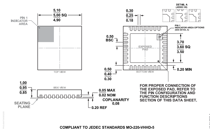
Figure 132. 32-Lead Lead Frame Chip Scale Package [LFCSP] 5 mm x 5 mm Body and 0.95 mm Package Height (CP-32-30) Dimensions shown in millimeters
