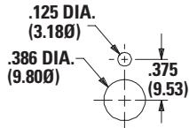
3/8 IN. BUSHING
