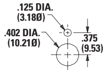
METRIC BUSHING
