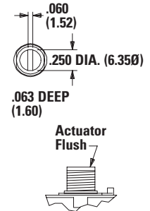
S1 Screwdriver Slot
