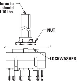
Typical Installation
