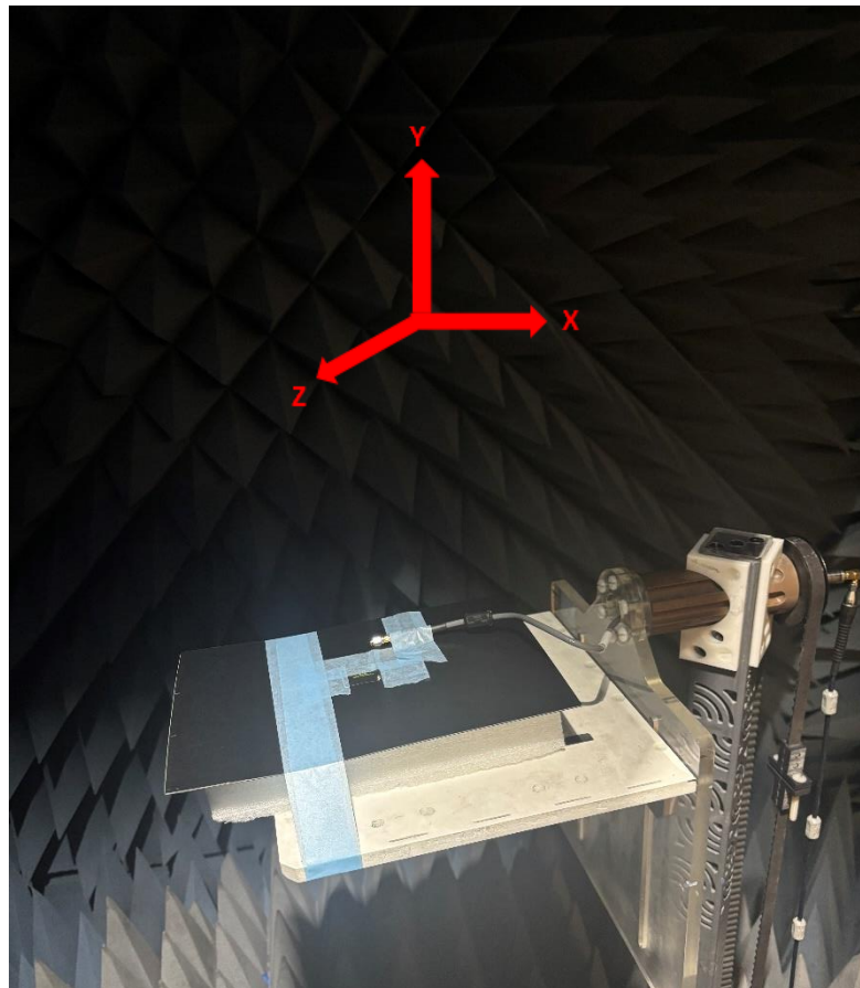
Chamber Test Set-up on 1mm ABS
