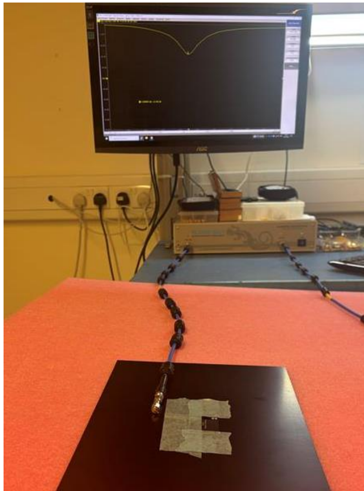
VNA Test Set-up on 1mm ABS
