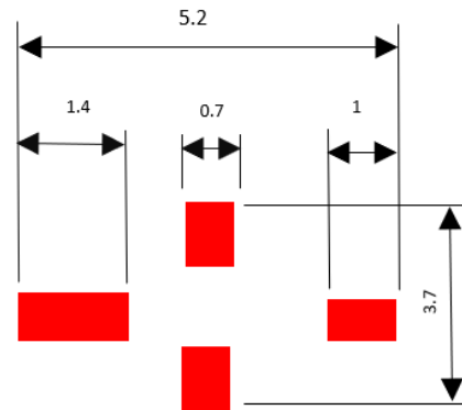
PCB Footprint
