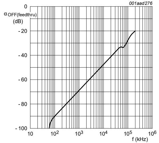
Fig. 13. Switch OFF-state signal feed-through as a function of frequency
