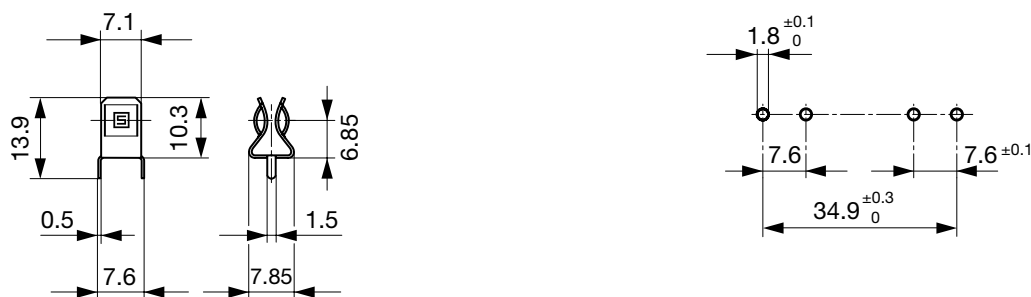
Drilling diagram
