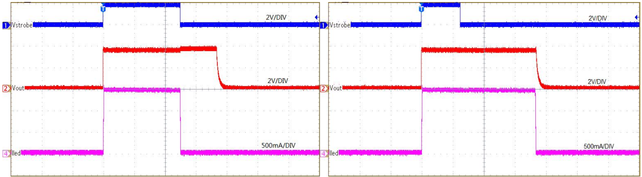
Time (40 ms/DIV)
