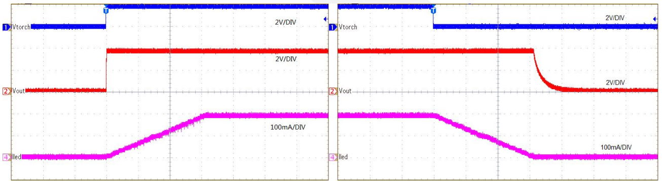
Time (10 ms/DIV)
