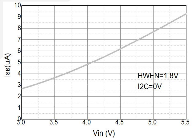
Figure 16. Standby current vs. Input voltage
