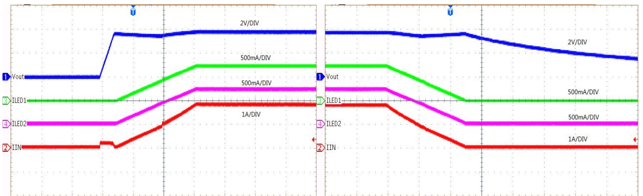
Time (400 us/DIV)
