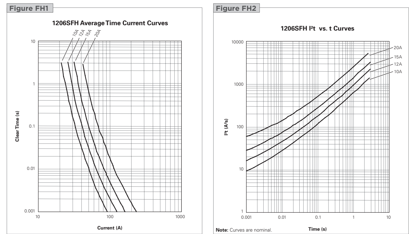
Figures FH1-FH2 Family Performance Curves for High-Current-Rated Chip Fuses
