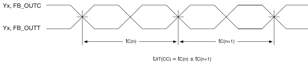
Cycle-to-Cycle Jitter
