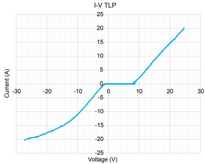
Figure 24. TLP characteristic
