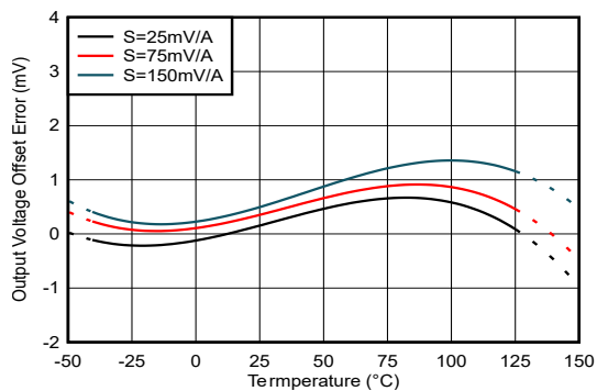
Figure 6-3. Offset Error vs Temperature: TMCS1133Bxx Device Options
