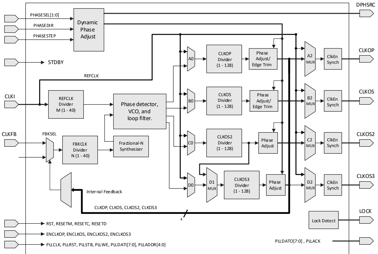
Figure 2.6. PLL Diagram
