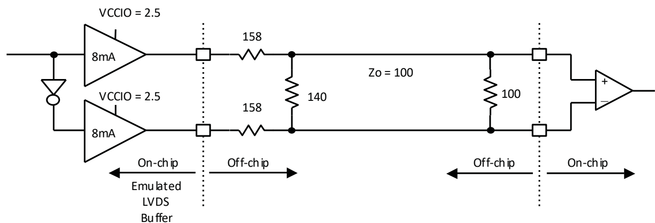
Figure 3.1. LVDS Using External Resistors (LVDS25E)
