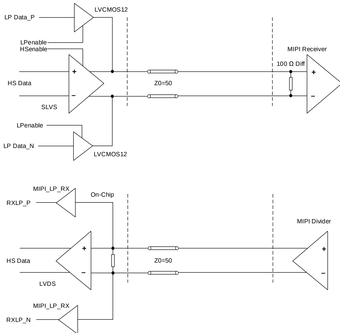
Figure 3.6. MIPI Interface
